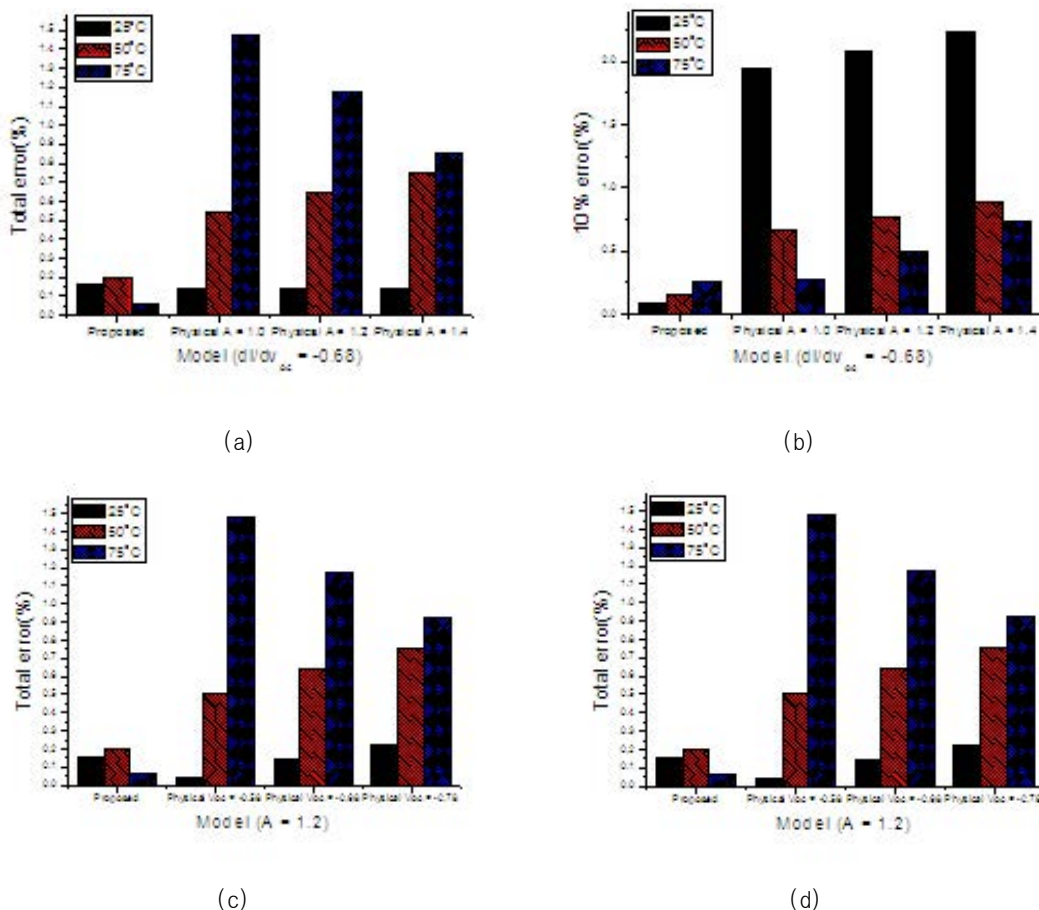
Fig. 10. Model accuracy under varying temperature.
