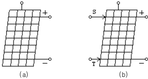
Fig. 1. PSIM solar model. (a) functional. (b) physical.
